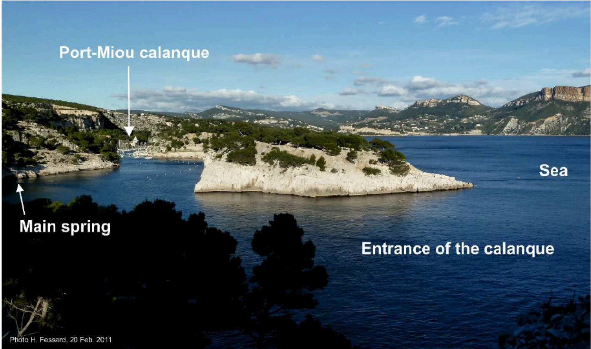
A 1: Panoramic view of the Port-Miou calanque (Cassis, SE France).
