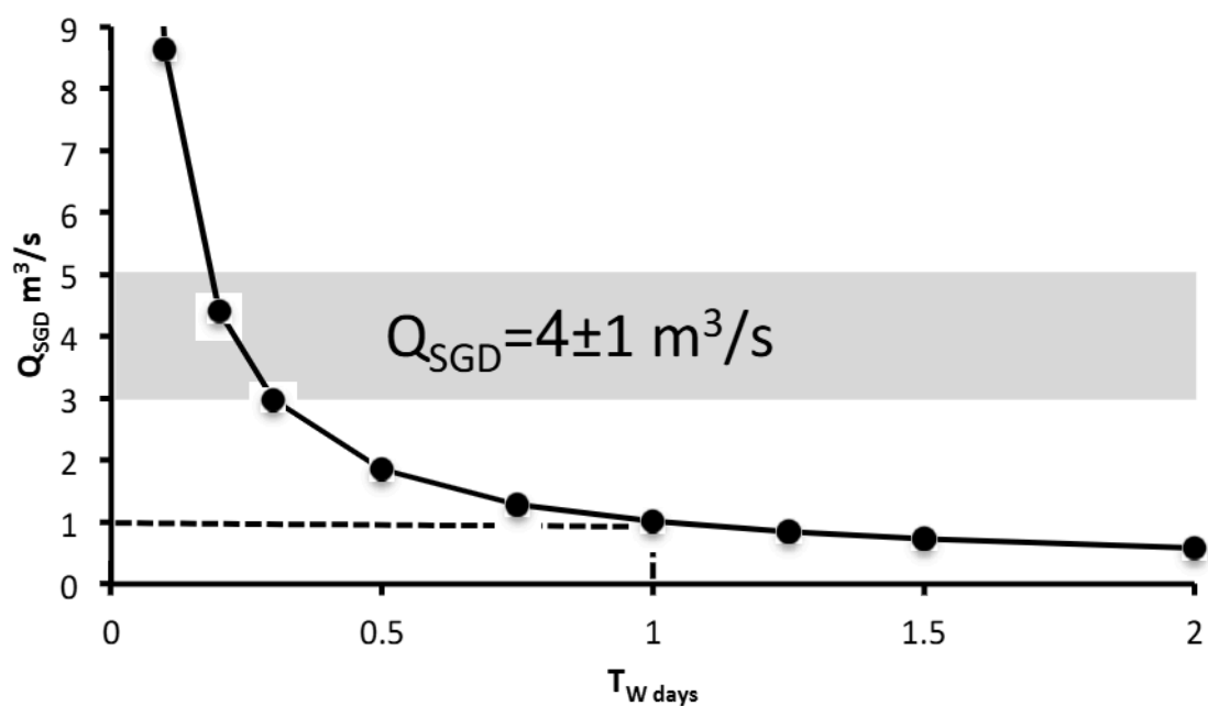
858 859 Figure 8: Simulation of Q_{SGD} calculated using ^{224}\text{Ra} measurements against the water residence 860 time. The grey bar refers to the Q_{SGD} measured during the sampling period ( 4 \pm 1 \text{ m}^3/\text{s} ). 861
