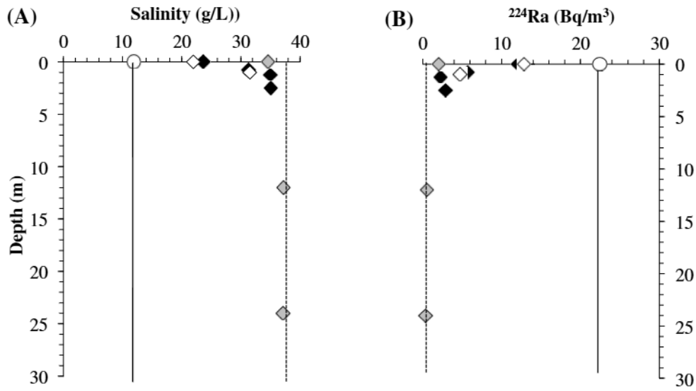
Figure 5: Salinity (A) and ^{224}\text{Ra} (B) against depth at the location of PM7 (2012) and at the location of PM_Cap in January 2013 and August 2014. The black dotted line at 38 g/L and 0.4 Bq/m 3 for salinity and ^{224}\text{Ra} respectively, indicates the seawater value. The black line at 10 g/L and 22 Bq/m 3 for salinity and ^{224}\text{Ra} respectively, indicates the value of the karstic spring. Error bars are smaller than the symbols. The symbols are the same as in Fig. 4.
