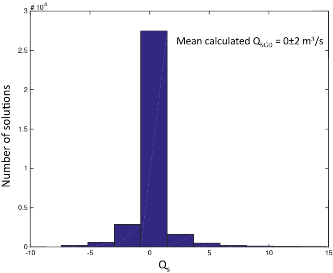
855 856 Figure 7: Solutions for Q_{SGD} according to the system of 3 equations based on the data 857 collected in 2014. Q_{SGD} measured during the same period of time is 4 \pm 1 \text{ m}^3/\text{s} .
