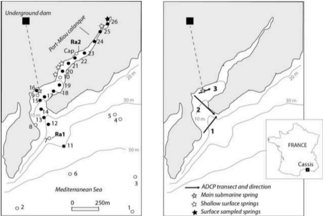
Figure 1: Location map and numbers (#) of samples (hereafter labelled PM#) collected in the Calanque of Port-Miou in 2012 and 2014. Ra1 and Ra2 are the radium depth
