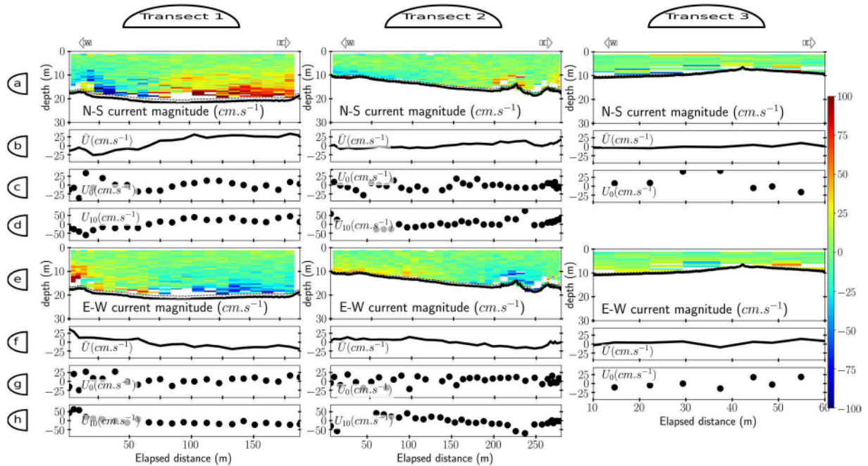
Figure 6: Selected transects (T1: entrance of the calanque, T2, within the calanque, and T3: above the spring) depicting in a): the NS current magnitude profiles, b): the depth-averaged
