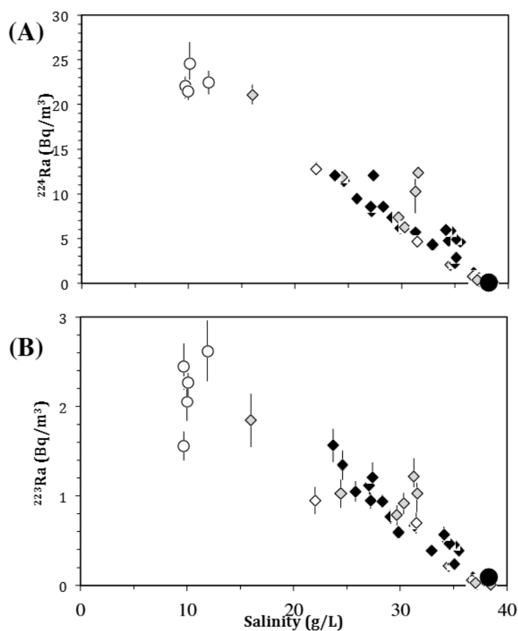
835 836 Figure 4: (A) ^{224}\text{Ra} and (B) ^{223}\text{Ra} against salinity in the Port Miou main karstic spring (open 837 circles), the surface waters and the depth profiles Ra1 and Ra2 in the calanque of Port-Miou. 838 Error bars are 1\sigma . Black diamonds are data collected in 2014, gray diamonds are data 839 collected in 2012, open diamonds are data collected in 2013. The black circle indicates the 840 value of coastal seawater.
